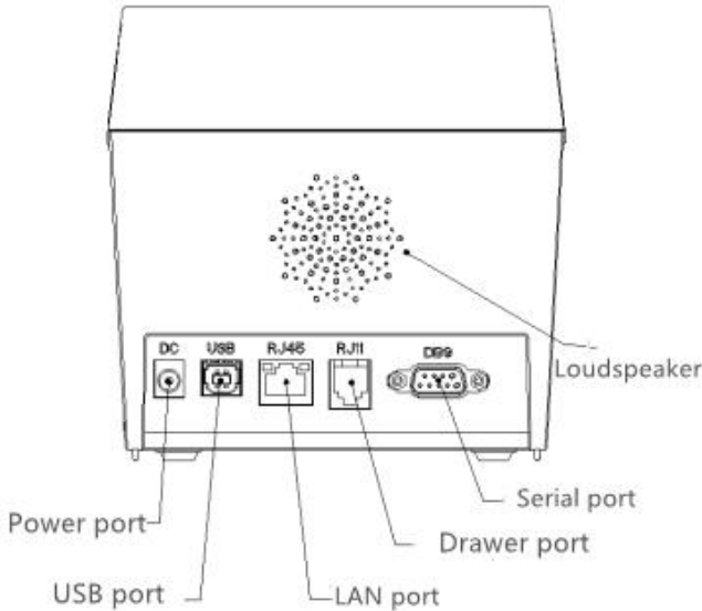
Figure 2-1 The name of each part of the printer
