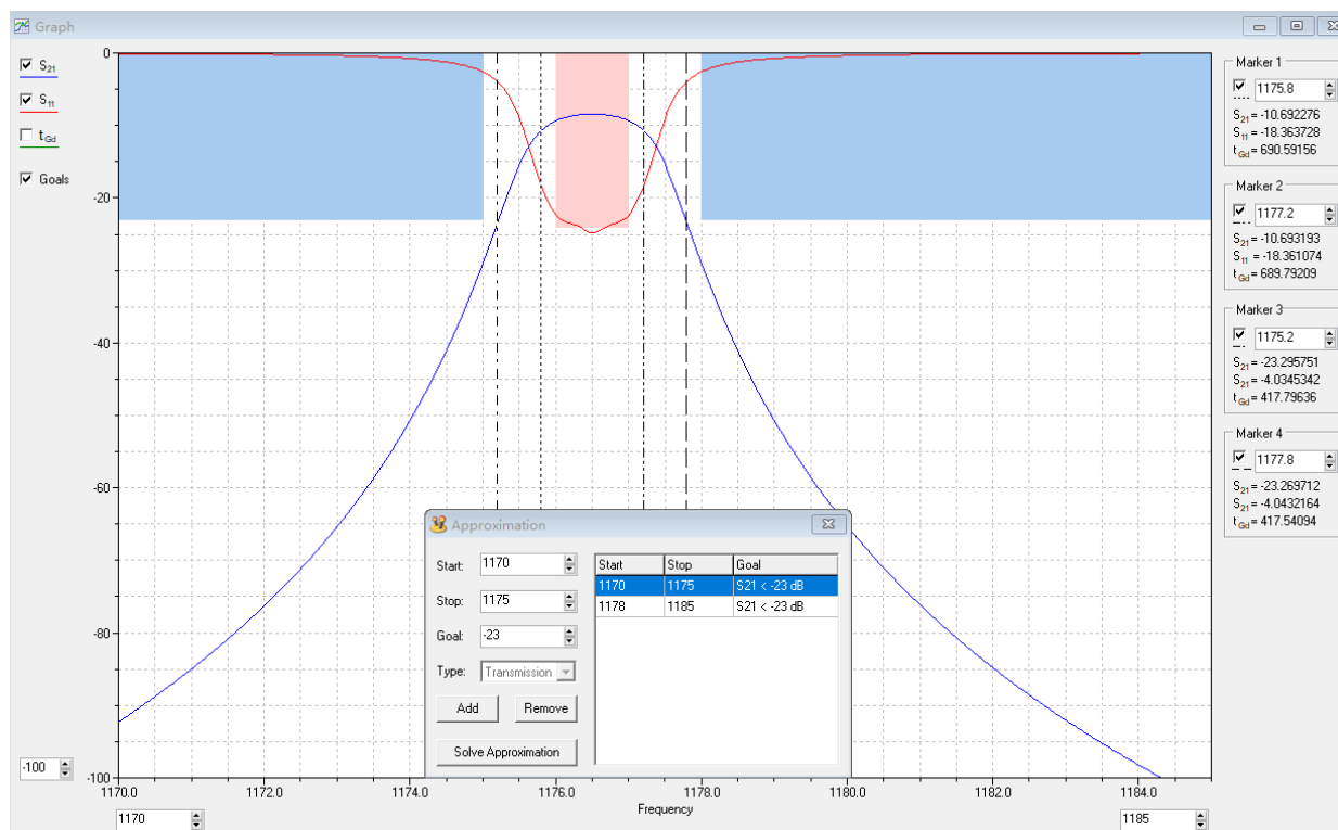
Figure 2 The simulation curve of the Filter
