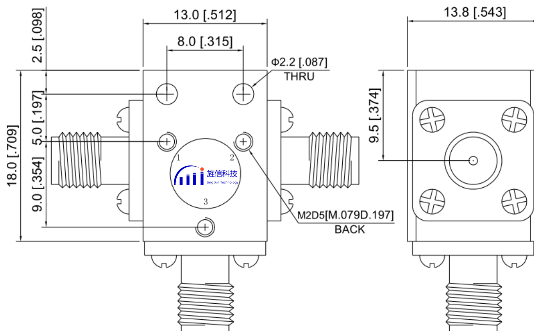
Figure 1 JX-CT-14G18G-17S front panel layout
