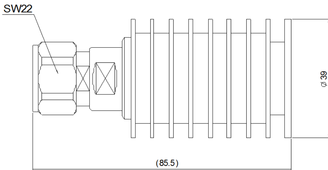
Figure 1 JX-PL-DC3G-4310M20W front panel layout
