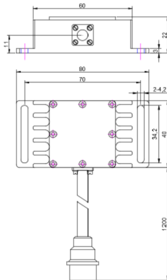
Figure 1 JX-AL-380-50W front panel layout
