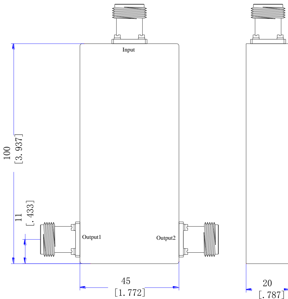
Figure 1 JX-PD-800M3800M-2N front panel layout
