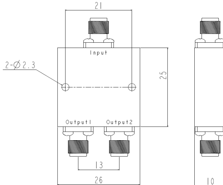
Figure 1 JX-PD2-27.5G29.5G-16F front panel layout
