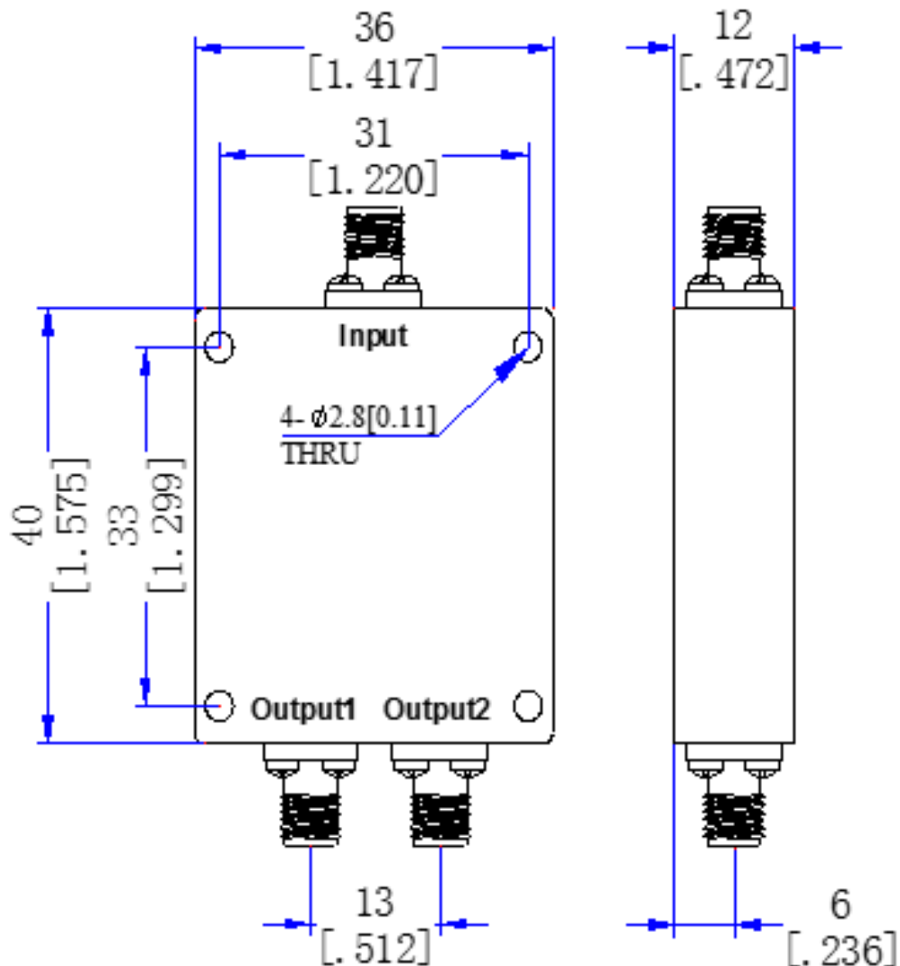
Figure 1 JX-PD1-700M2700M-20S-1
