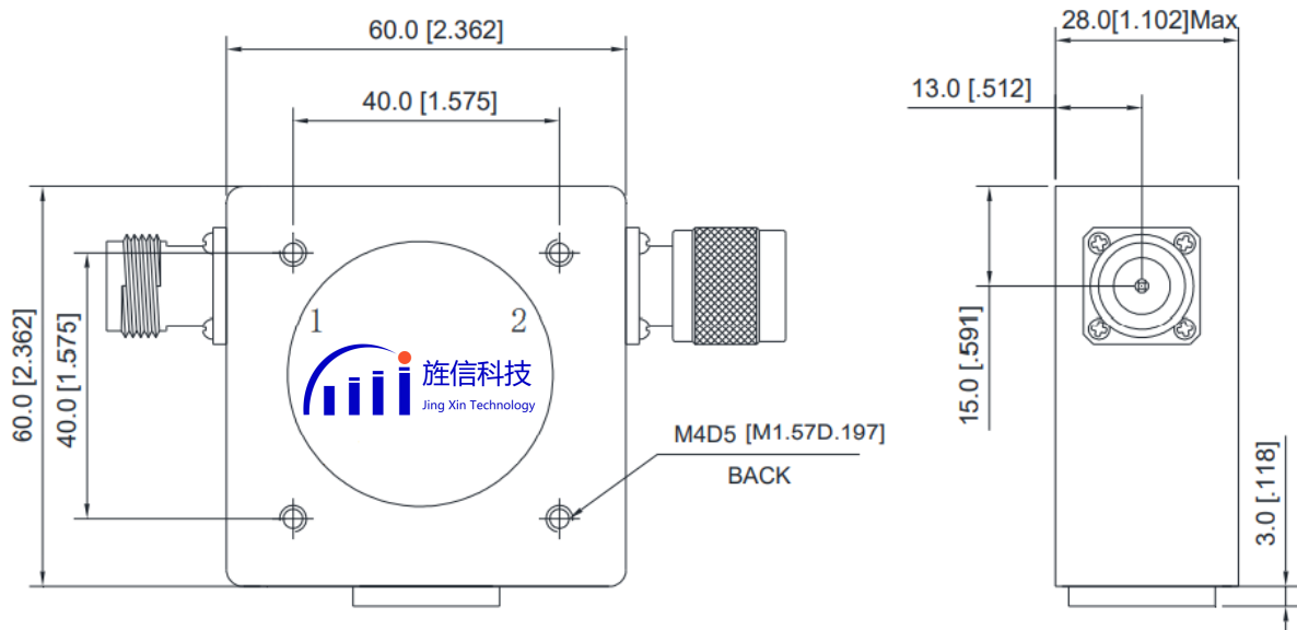
Figure 1 JX-CI-148M150M-60NF front panel layout
