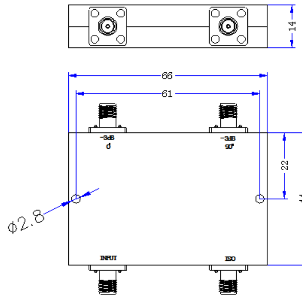
Figure 1 JX-BRIDGE3-136M240M-20S front panel layout
