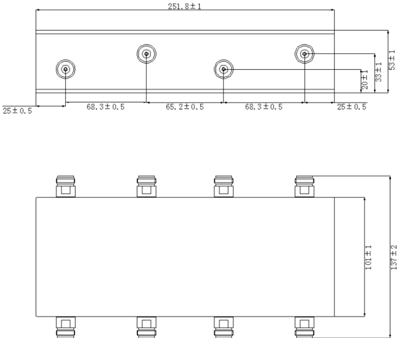
Figure 1 JX-BC4X4-380M2700M-NF front panel layout
