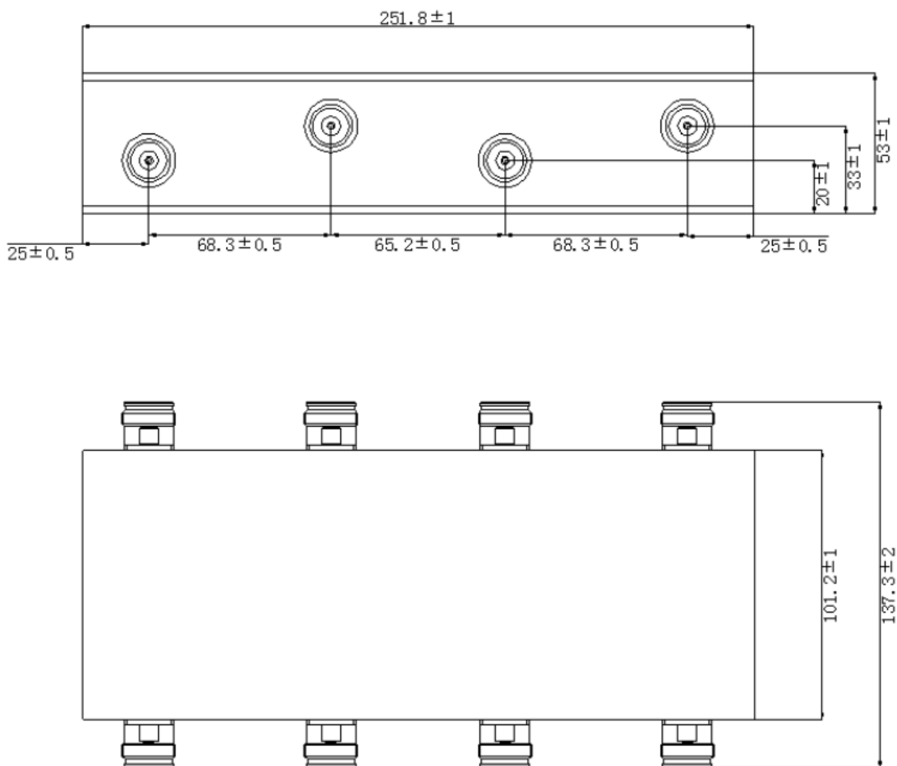
Figure 3 JX-BC4X4-380M2700M-4310F front panel layout
