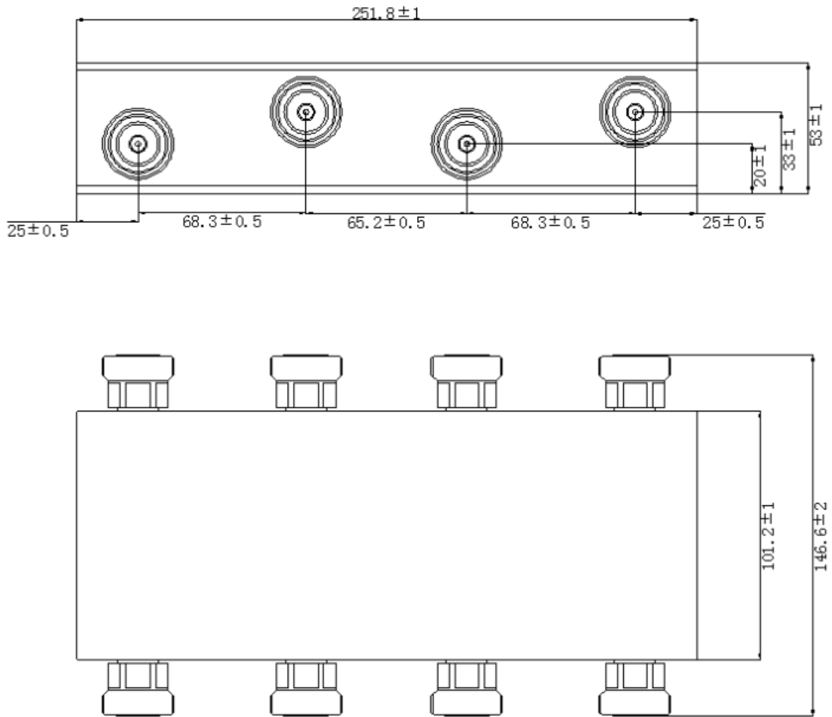
Figure 2 JX-BC4X4-380M2700M-DINF front panel layout
