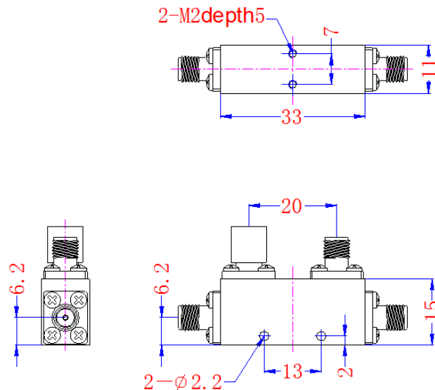
Figure 1 JX-DC-7.5G16G-S20 front panel layout
