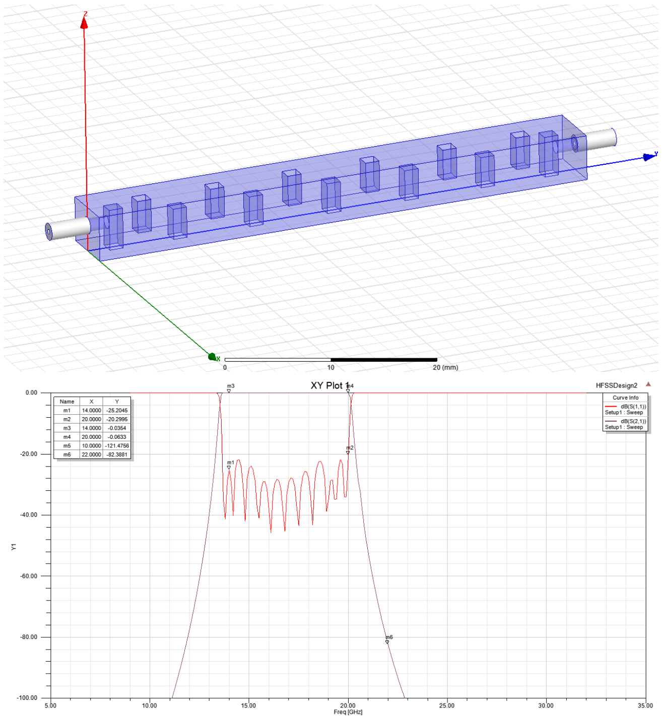
Figure 2 The simulation curve of the Filter
