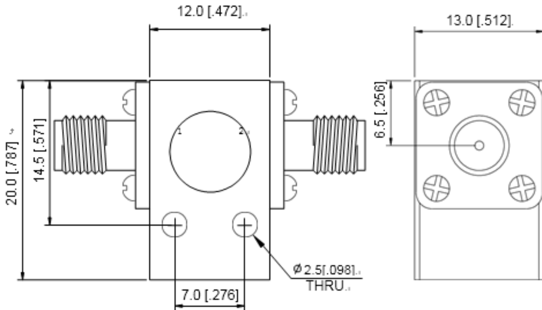
Figure 1 JX-TI-16G17G-23S front panel layout
