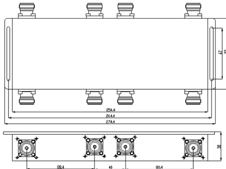
Figure 1 JX-BC4X4-698M2700M-4310F150 front panel layout
