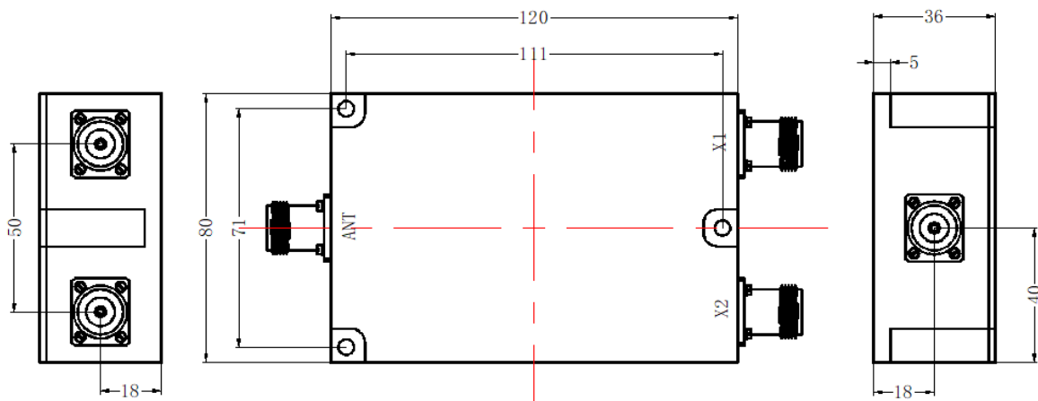
Figure 1 JX-LCC2-30M400M-20N front panel layout
