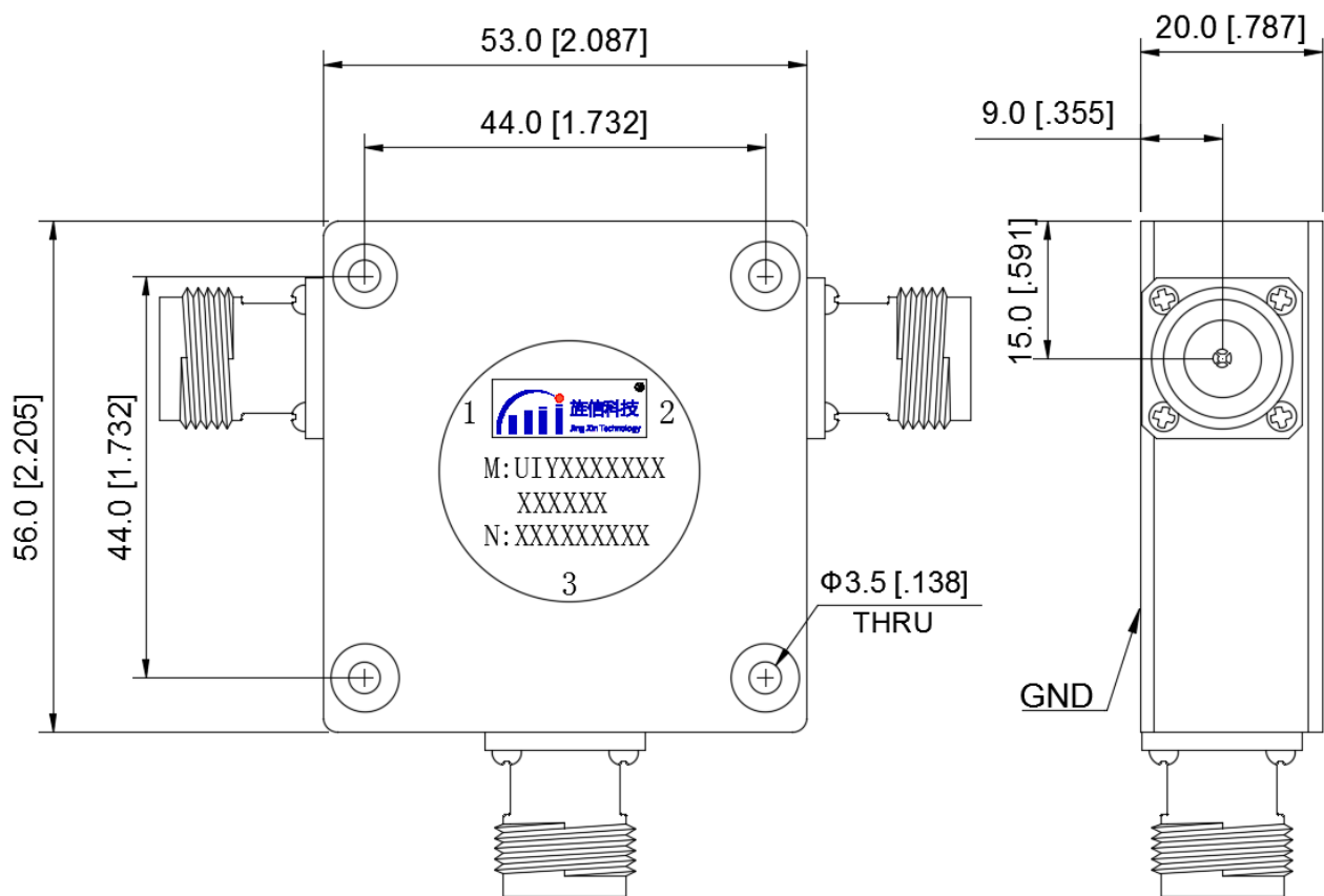
Figure 1 Circulator front panel layout
