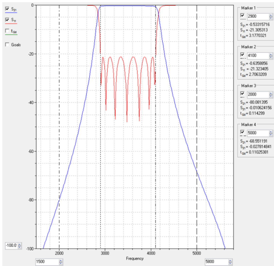
Figure 2 The curve of the Filter
