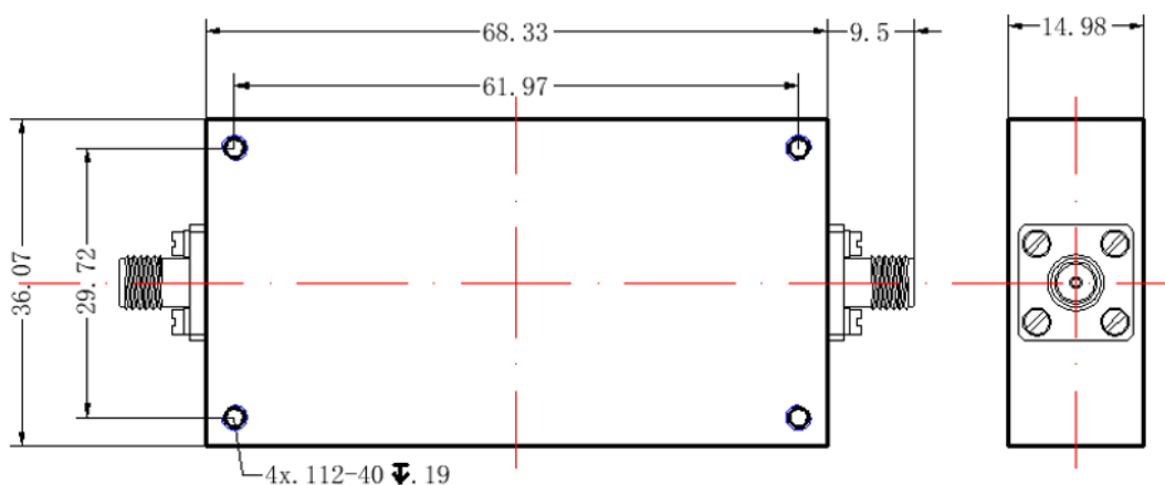
Figure 1 JX-CF1-2900M4100M-66S front panel layout
