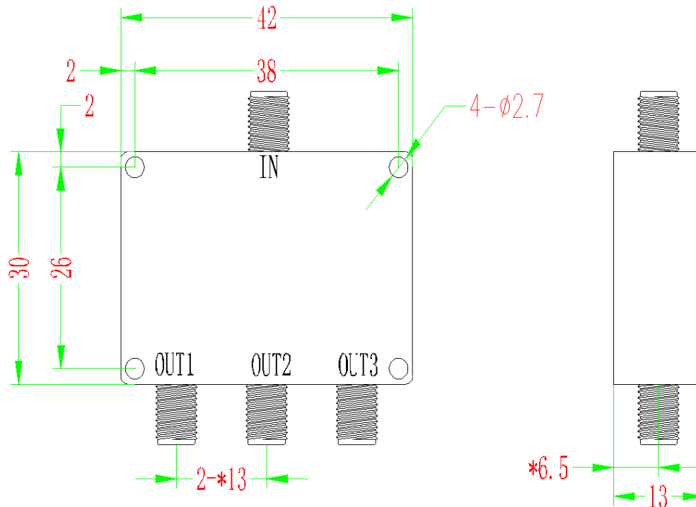
Figure 1 JX-PD3-10M500M-18S front panel layout
