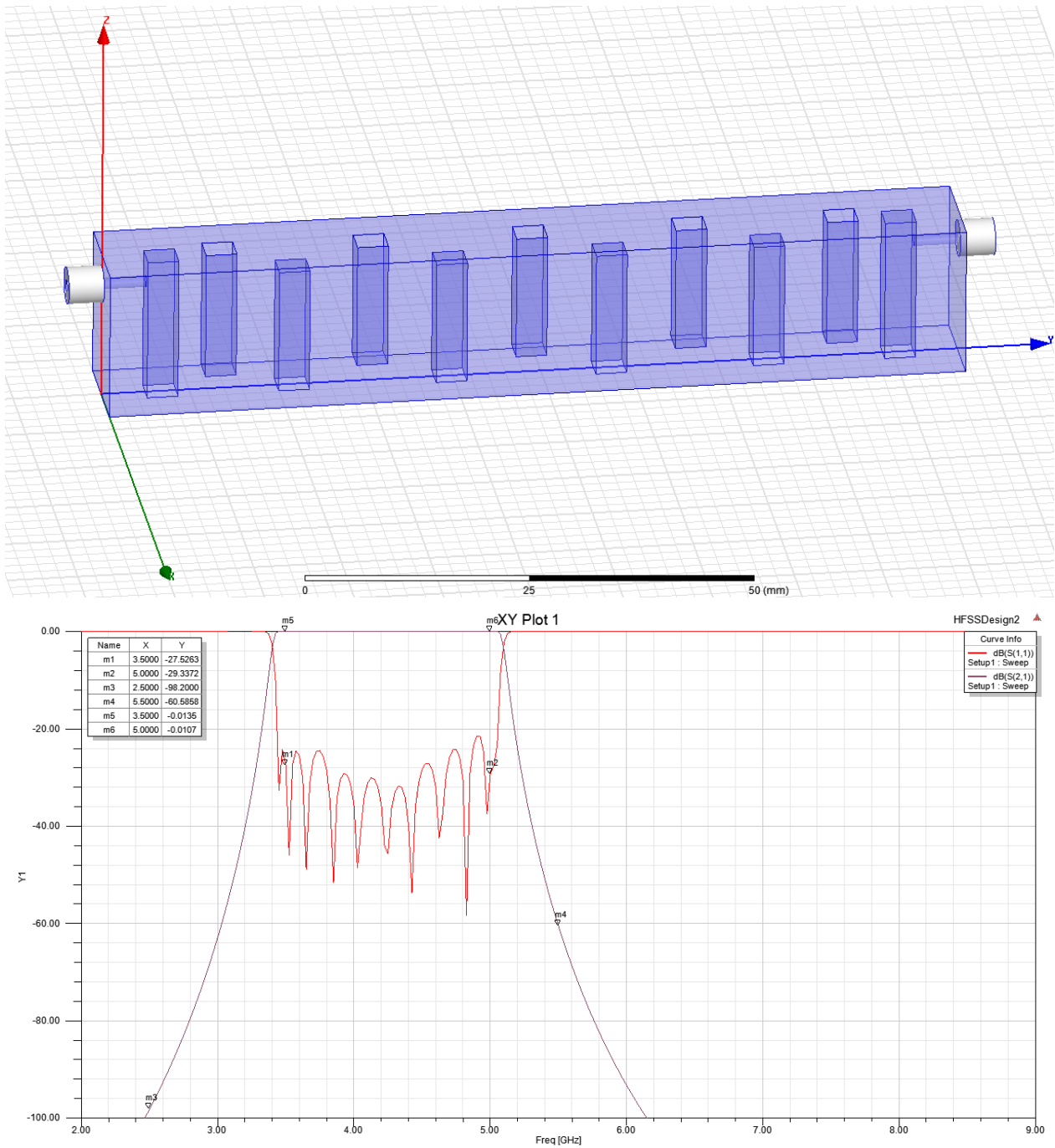
Figure 2 The simulation curve of the Filter
