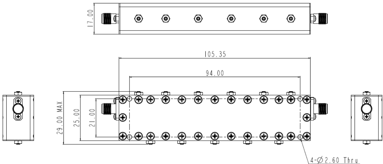
Figure 1 JX-CF1-35005000-11J front panel layout
