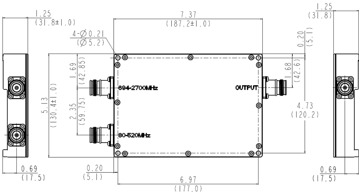
Figure 1 JX-CC2-BK24-4310FWP front panel layout
