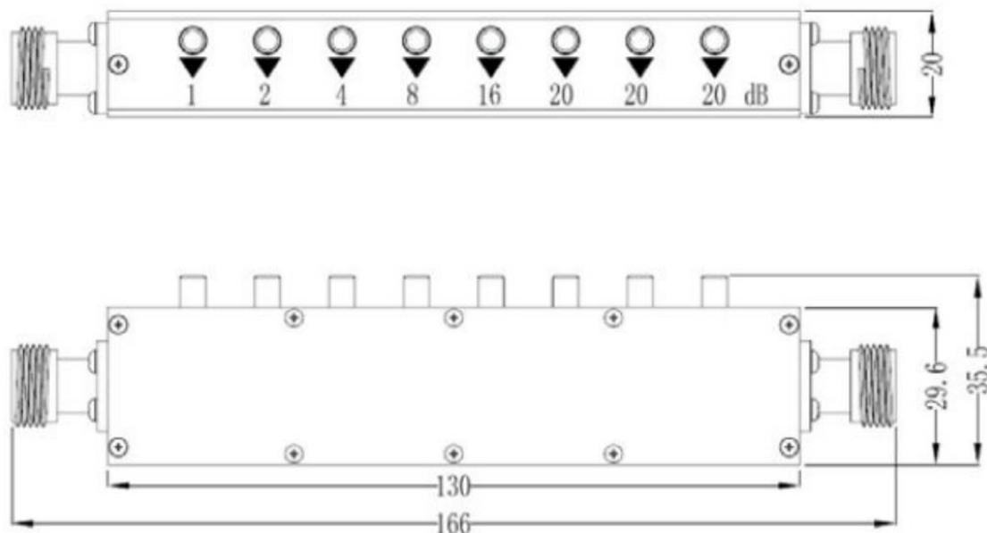
Figure 1 JX-AT-DC2.5G-5N91 front panel layout
