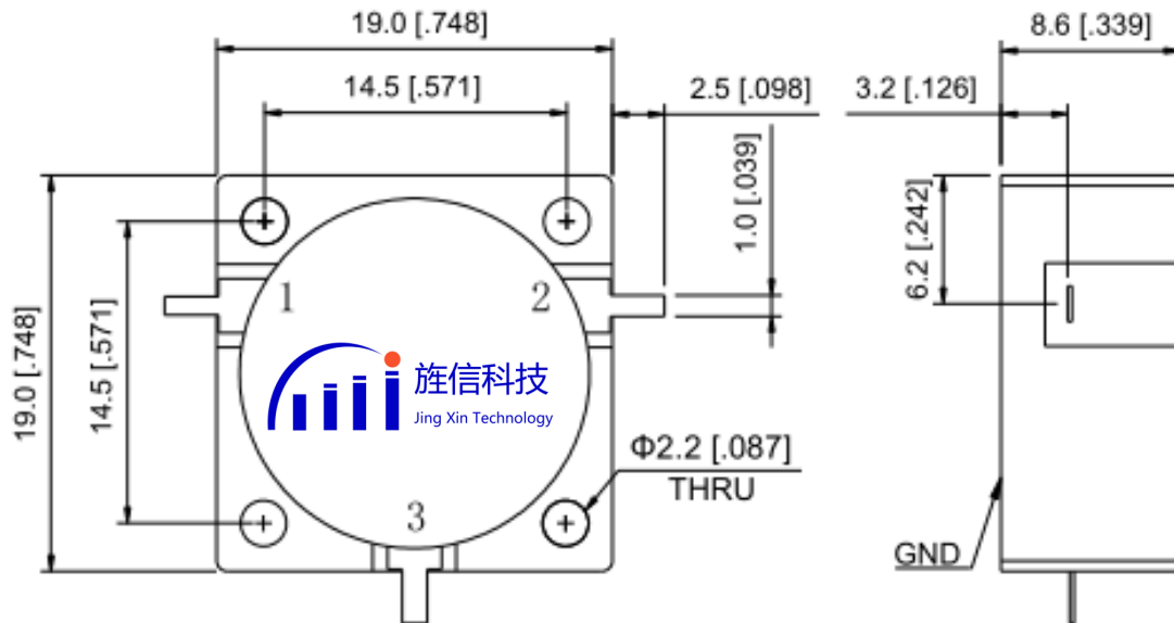
Figure 1 JX-CT-xxxMxxxM-xT front panel layout
