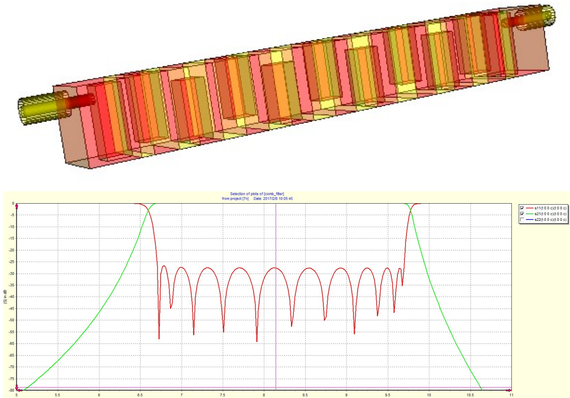
Figure 3 The simulation curve of Filter
