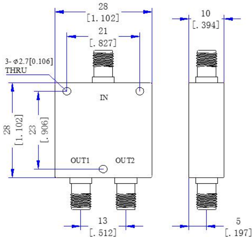
Figure 1 JX-PD2-4G8G-20S front panel layout
