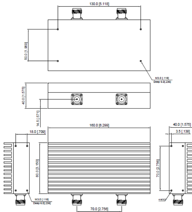
Figure 1 JX-CI1-380420-60N front panel layout
