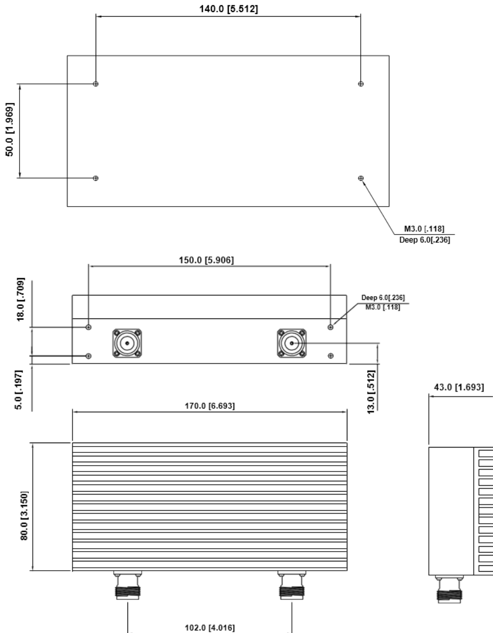
Figure 1 JX-CI1-146M174M-50N front panel layout
