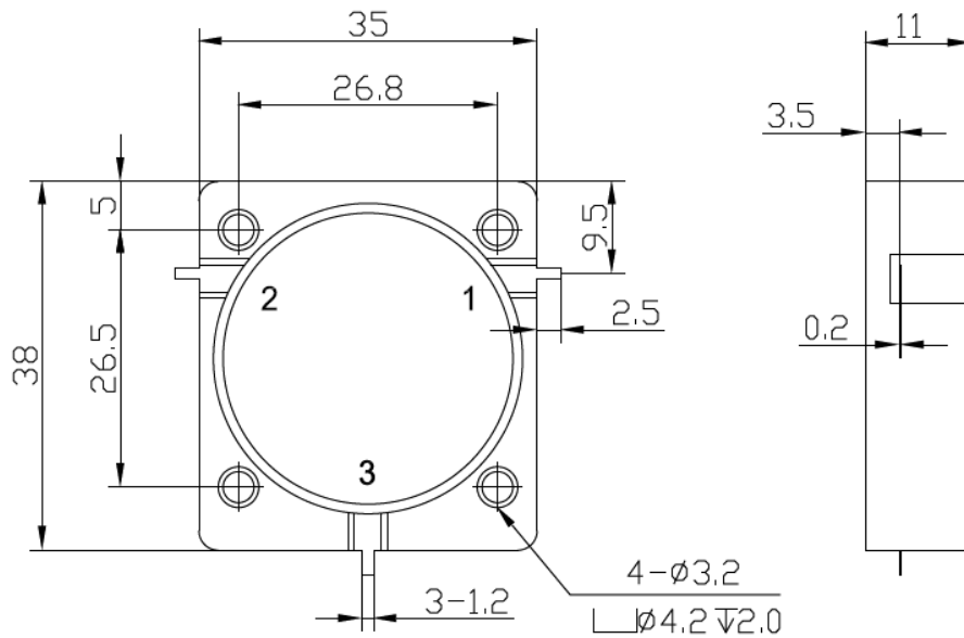
Figure 1 JX-TH-480-20-100M front panel layout
