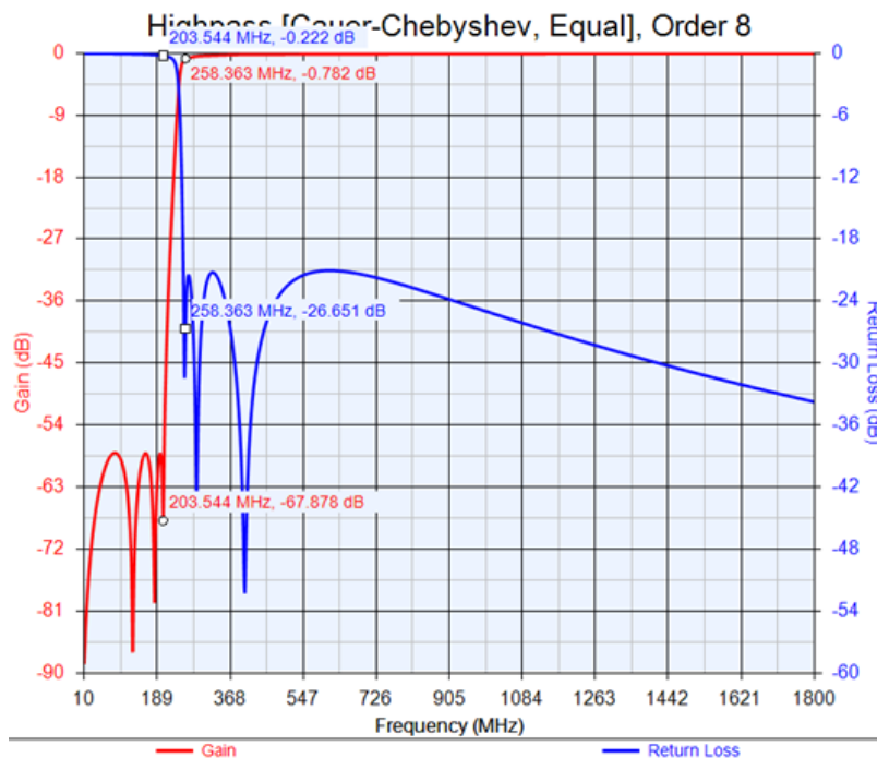
Figure 3 The simulation curve of the Filter
