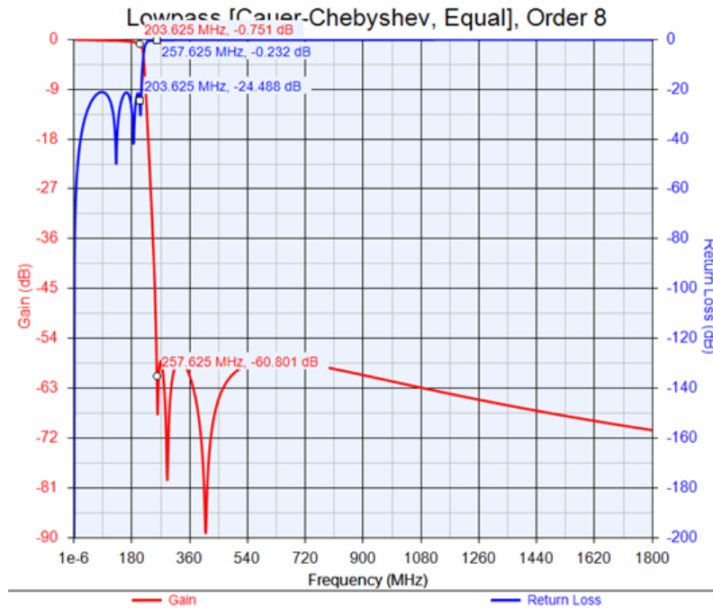
Figure 2 The simulation curve of the Filter
