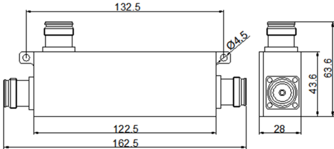
Figure 1 JX-PC-575-6000-XC43DI front panel layout
