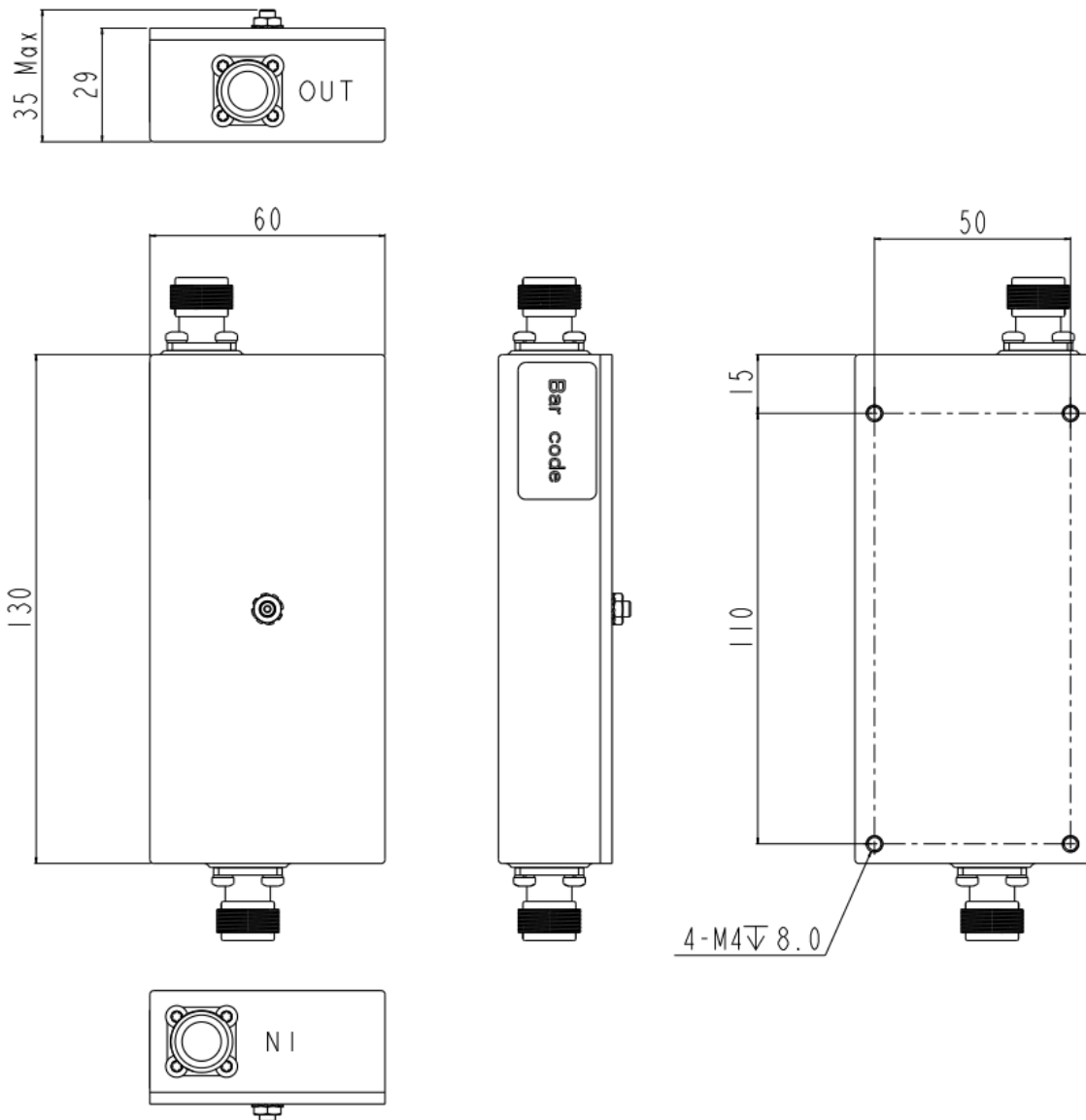
Figure 1 JX-CF1-1427M1518M-80N front panel layout
